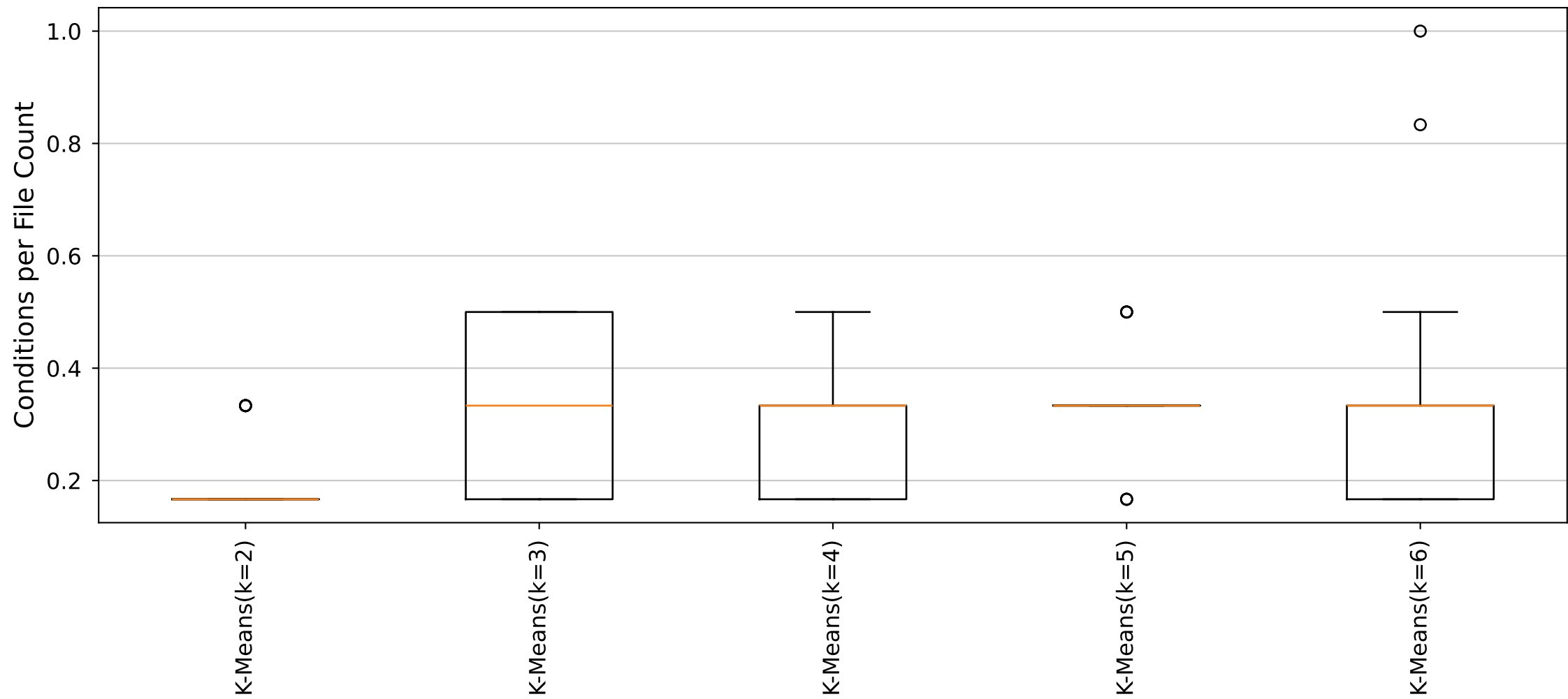
YARA Rules Conditions per File Count Distribution (Cluster24_Size6 dataset)
